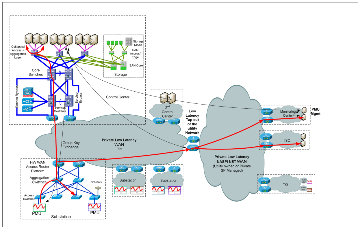
Figure 13.20. Example Synchrophasor Data Flows Across Multiple Networks
