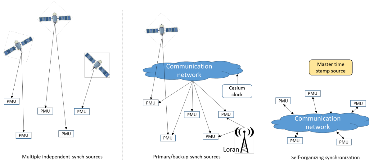
Figure 13.25. Structural Models for Timing Distribution
