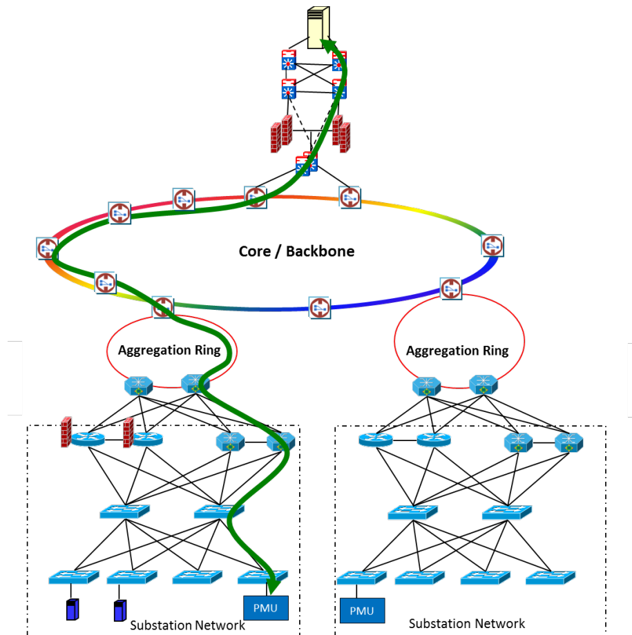
Figure 13.27. Two Substation PMU Data Flow Example
